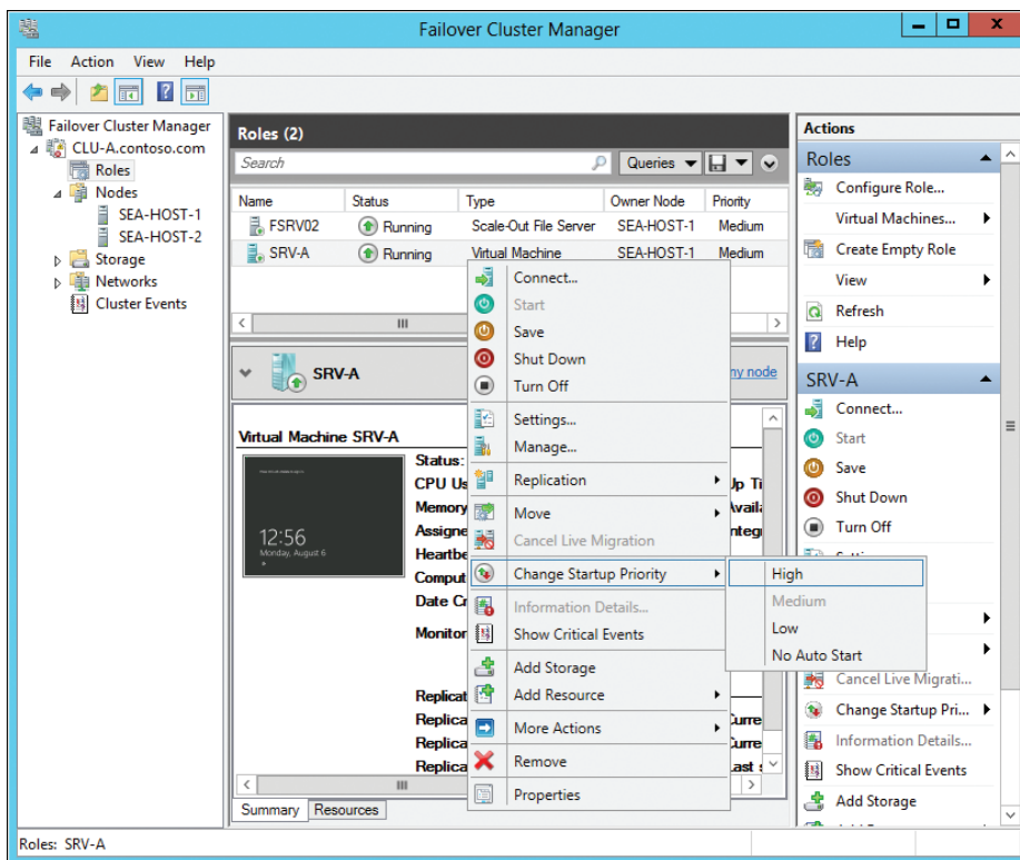
FIGURE 3-3 Using Failover Cluster Manager to configure the priority of a clustered VM.
