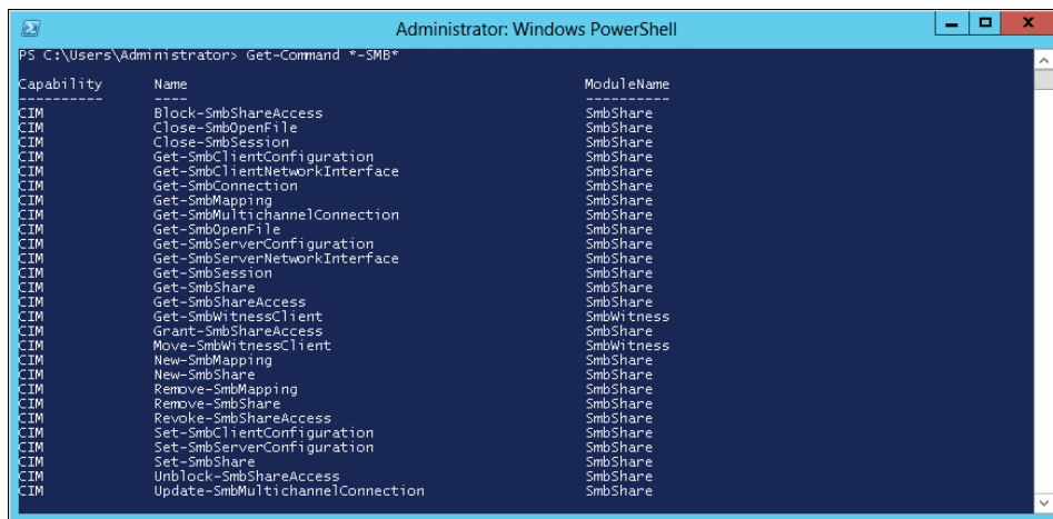
FIGURE 2-17 Windows PowerShell cmdlets for managing SMB features and infrastructure.
