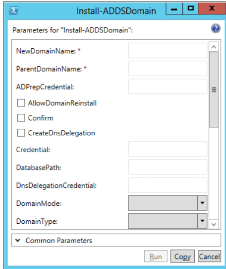
FIGURE 3-12 Example of using the Show-Command cmdlet.
